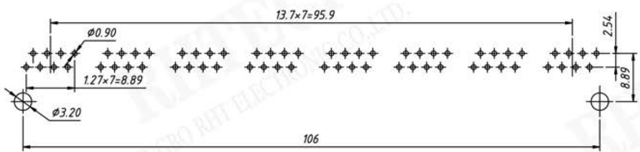
PCB Layout
