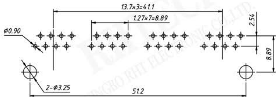
PCB Layout
